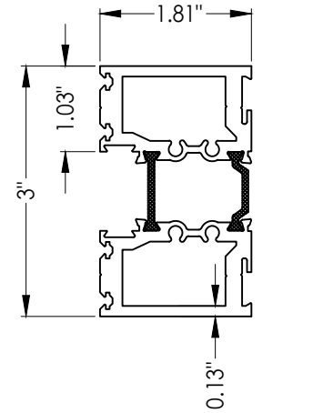
1 LT NARROW FRAME
