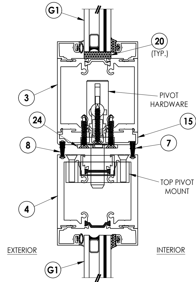
4 VERTICAL CROSS SECTION 4
